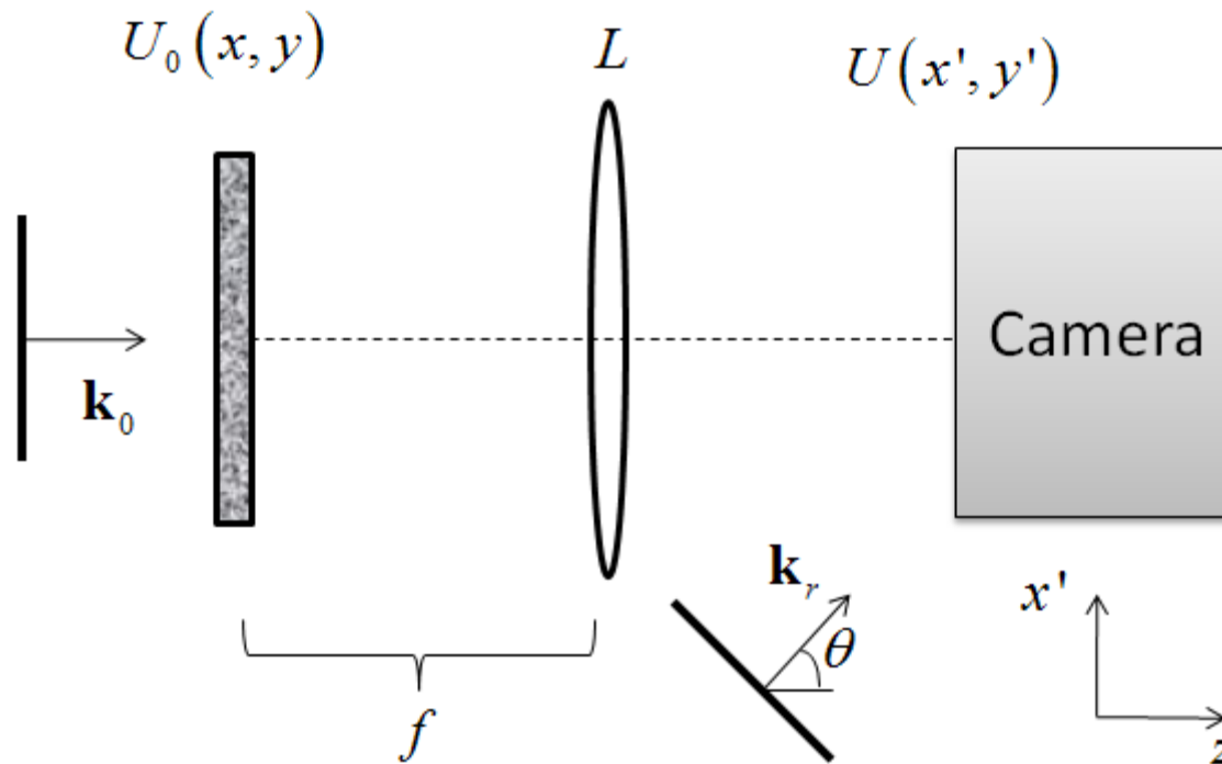
Figure 8. Digital recording of a Fourier hologram.
