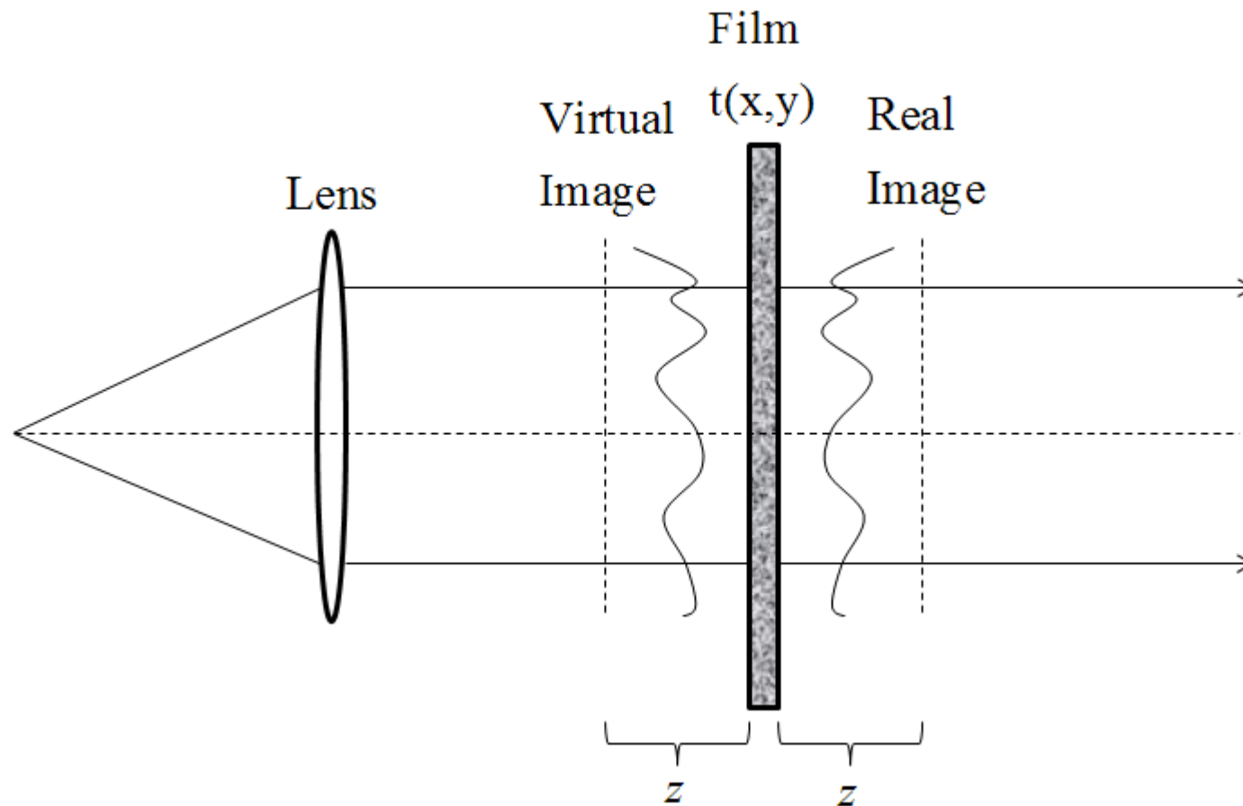
Figure 2. Reading an in-line hologram.
