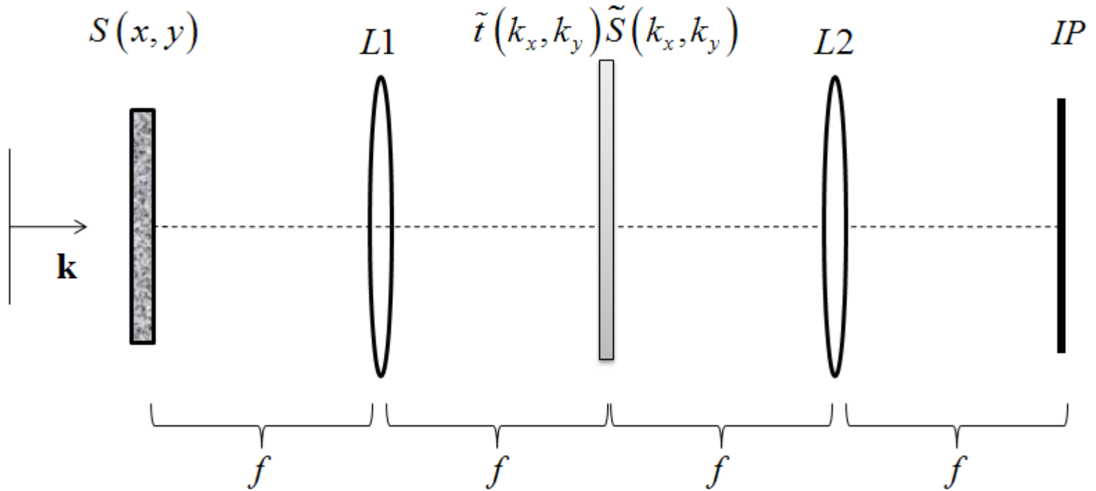
Figure 6. 4f optical system with digitally printed hologram, \tilde{t}(k_x, k_y) , in the Fourier plane; S(x, y) unknown signal, L1 , L2 lenses, IP image plane.
