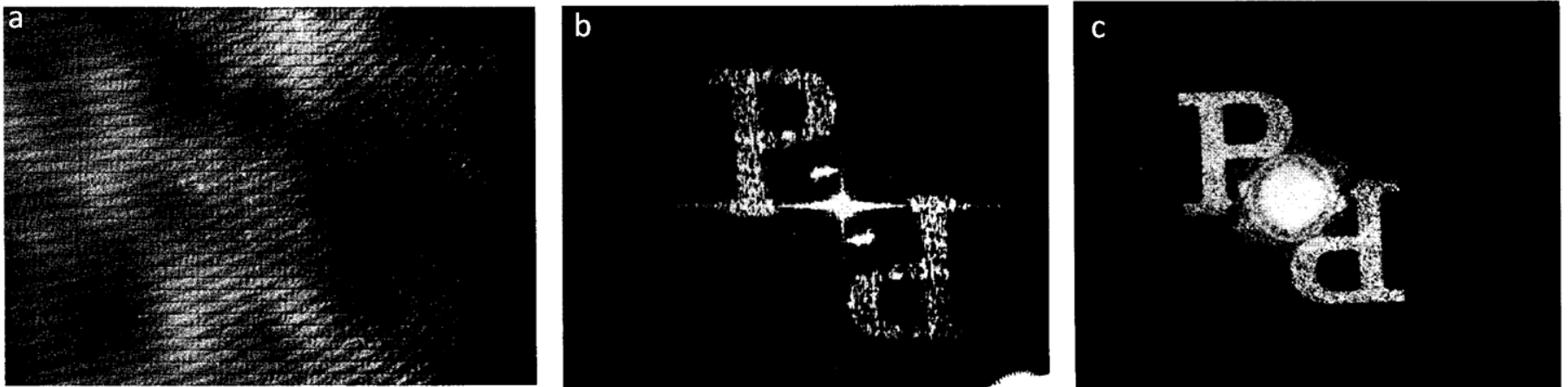
Figure 9. a) Hologram stored in computer memory; b) Display of the image reconstructed by digital computation; c) Image obtained optically from a photographic hologram, shown for comparison. Ref. [16].
