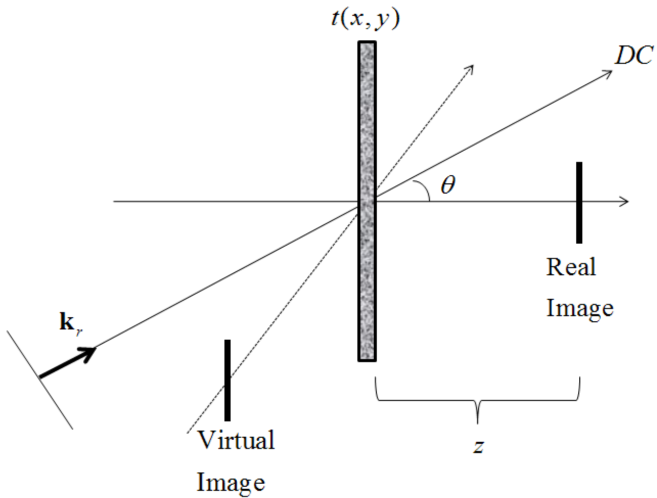
Figure 4. Reading the off-axis hologram.
