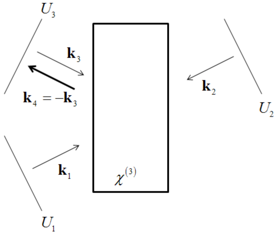
Figure 5. The four wave mixing process: emerging field U_4 is phase conjugated to U_3 .
