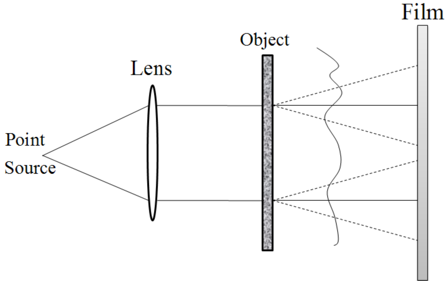
Figure 1. In-line optical setup for writing Fresnel holograms.
